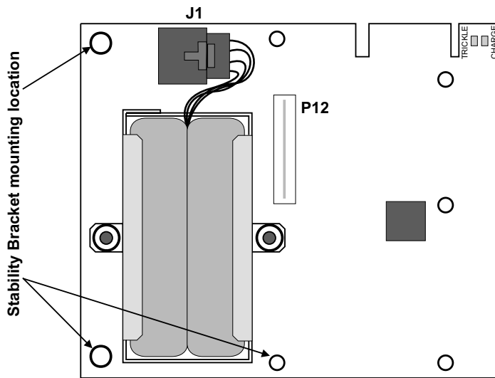
Board shown without Stability Bracket
