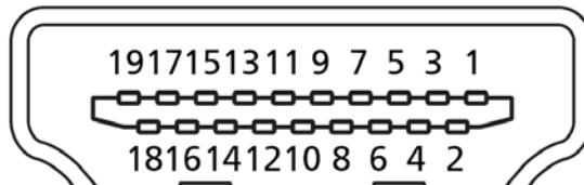
19-pin color display signal cable (Optional)
