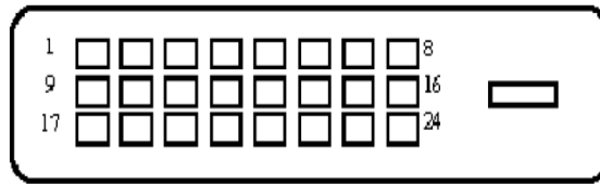
24-Pin Color Display Signal Cable
