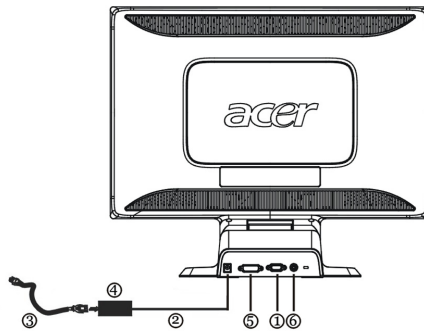
Figure 1 Connecting Cables
