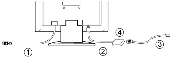
Figure 2 Connecting Cables
