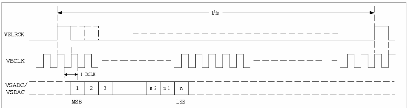
Figure 8. PCM MONO Data Mode A Format (bclk_polarity=1)
