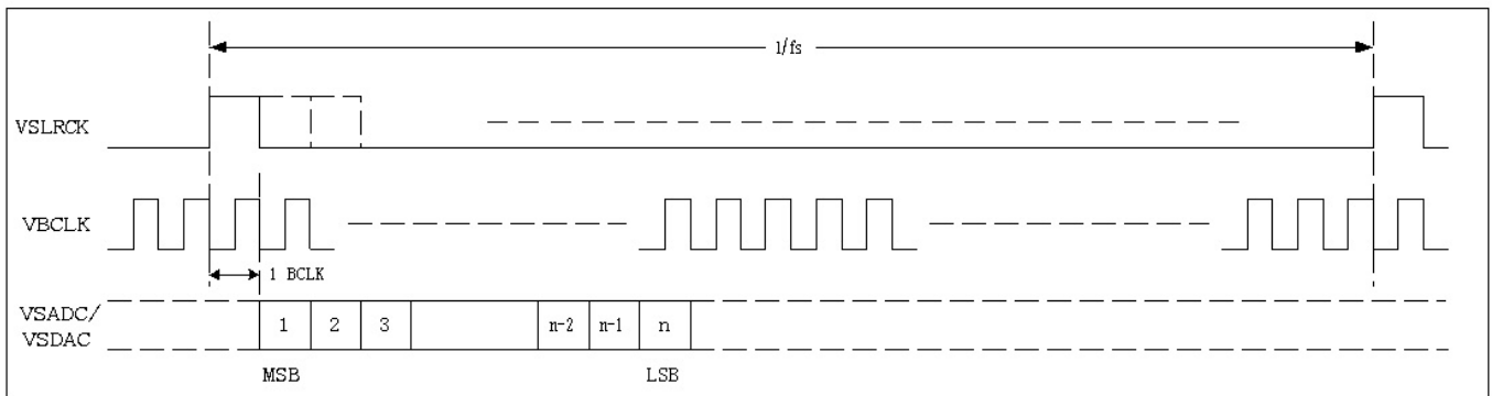
Figure 7. PCM MONO Data Mode A Format (bclk_polarity=0)
