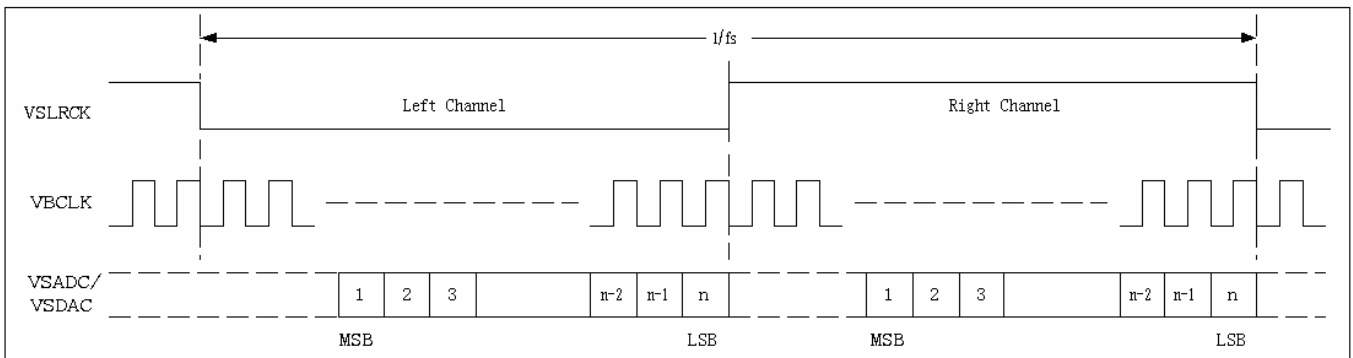
Figure 14. Right-Justified Data Format (bclk_polarity=0)
