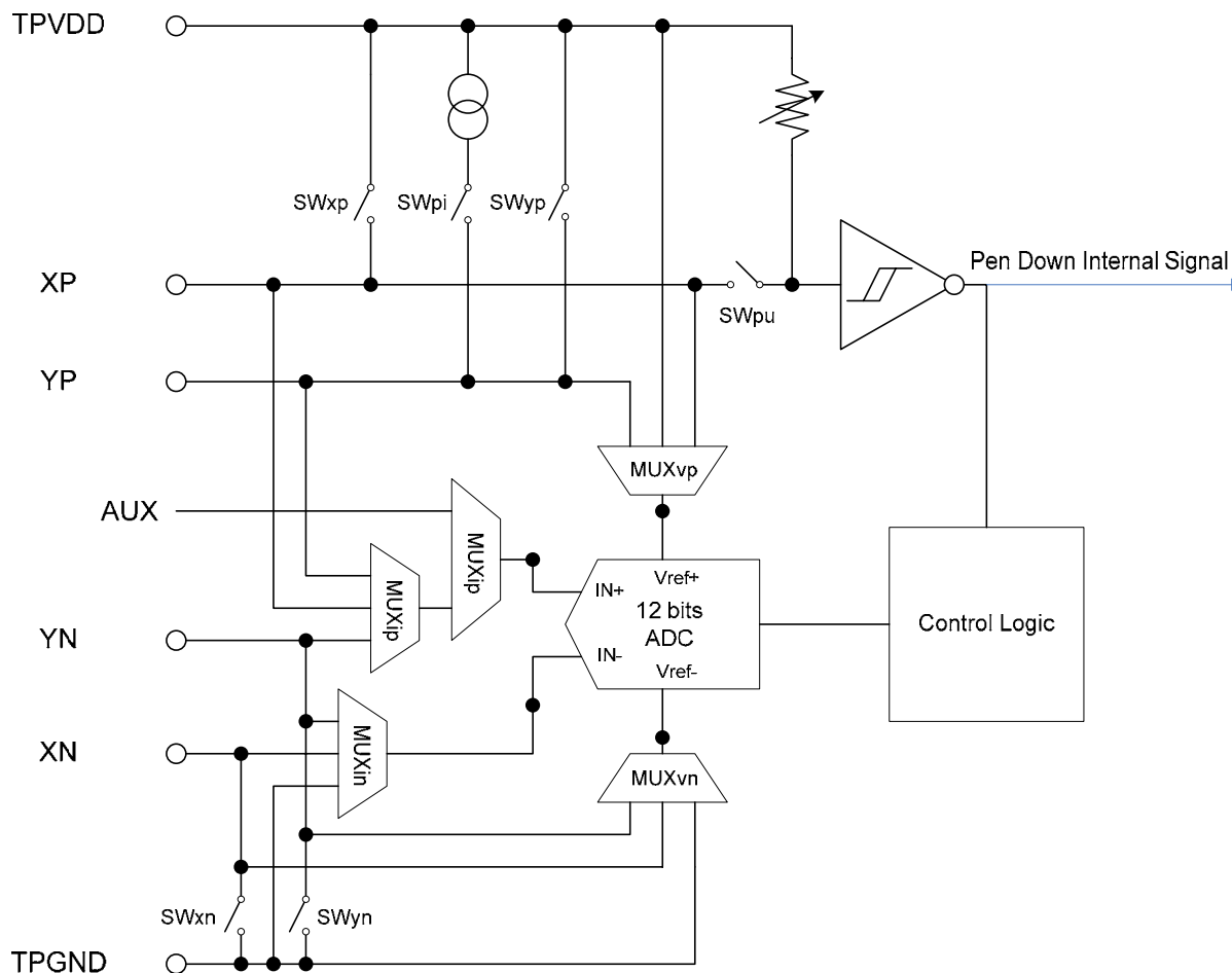
Figure 17. 4-Wire Resistive Touch Panel Circuit
