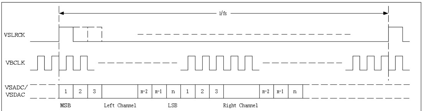
Figure 11. PCM Stereo Data Mode B Format (bclk_polarity=0)
