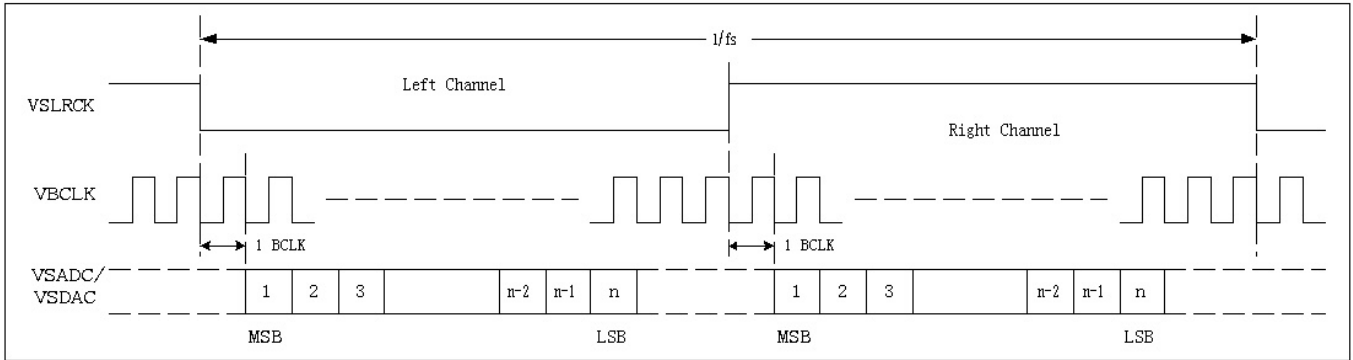
Figure 12. I 2 S Data Format (bclk_polarity=0)
