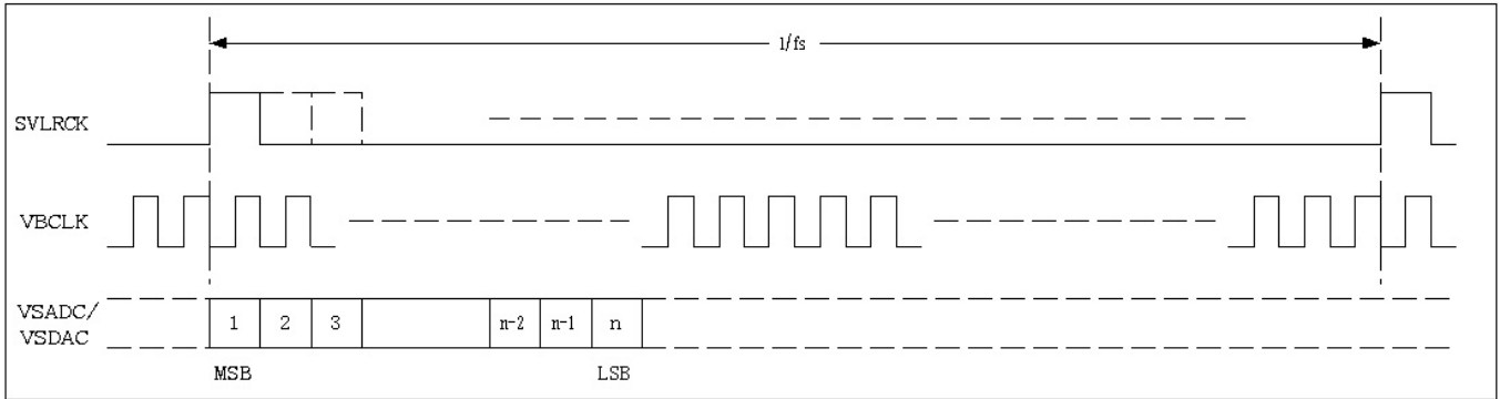
Figure 9. PCM MONO Data Mode B Format (bclk_polarity=0)
