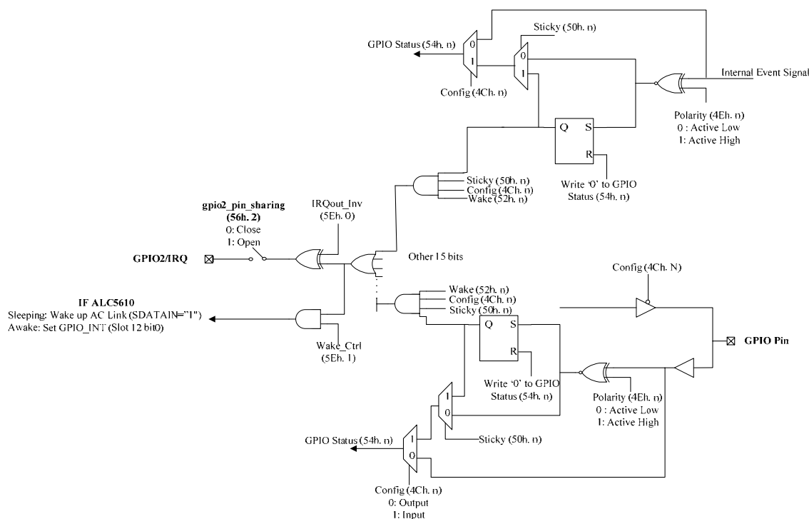
Figure 20. GPIO Implementation
