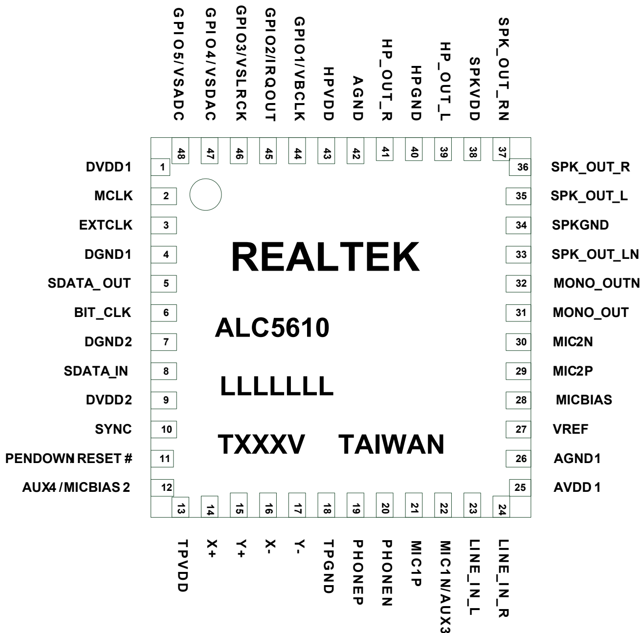
Figure 3. Pin Assignments
