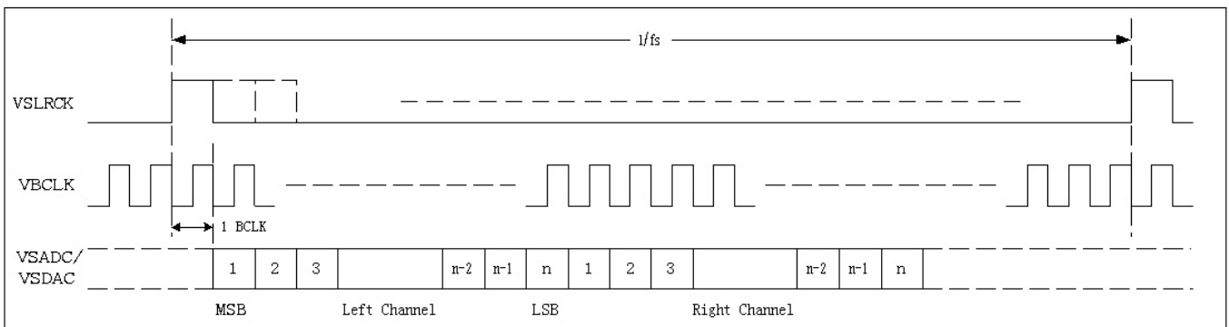
Figure 10. PCM Stereo Data Mode A Format (bclk_polarity=0)
