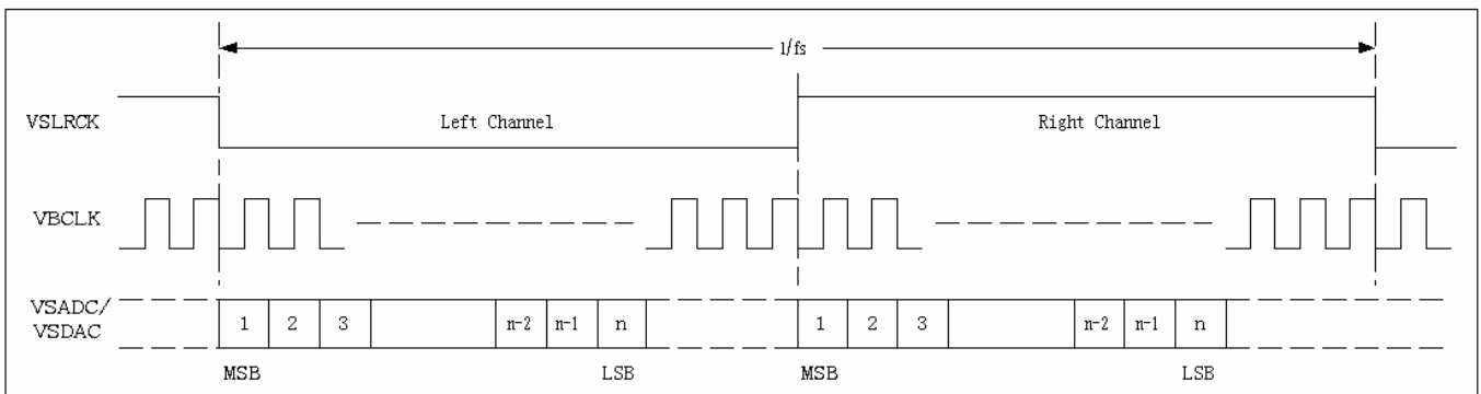
Figure 13. Left-Justified Data Format (bclk_polarity=0)
