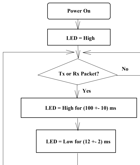
Figure 5. LED_TX+LED_RX
