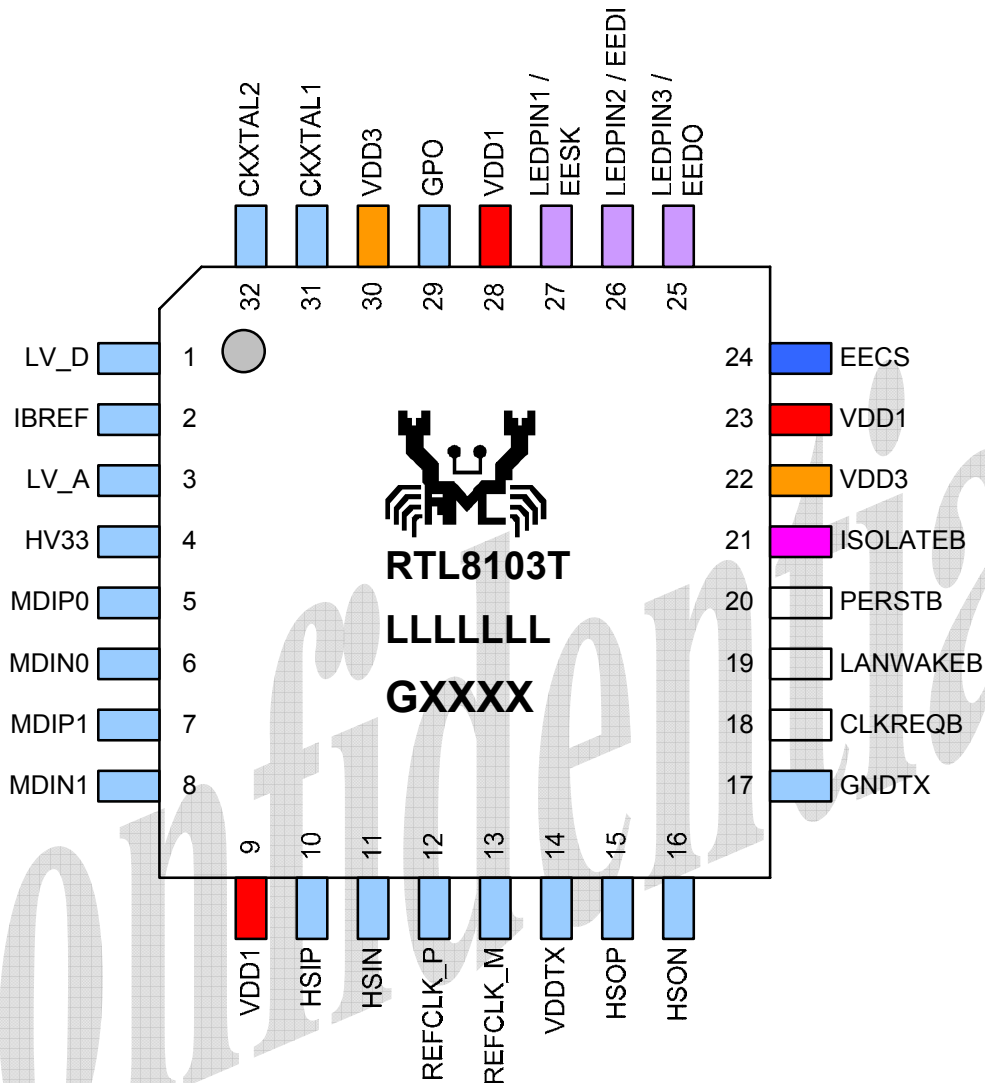
Figure 1. Pin Assignments
