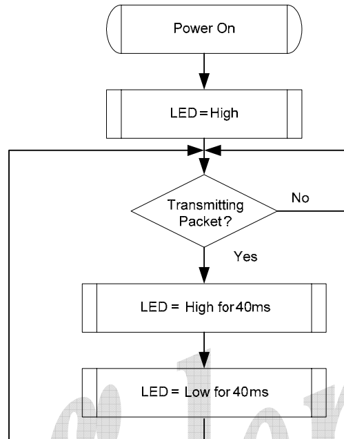
Figure 3. Tx LED
