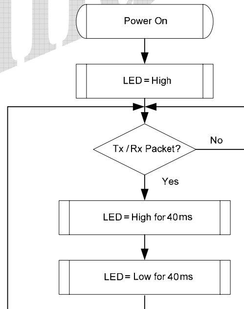
Figure 4. Tx/Rx LED
