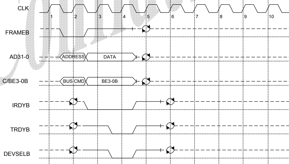
Figure 18. I/O Write
