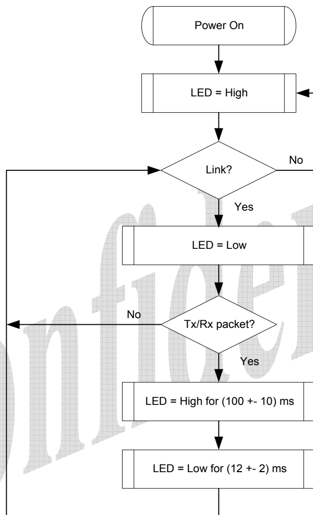
Figure 11. LINK/ACT LED
