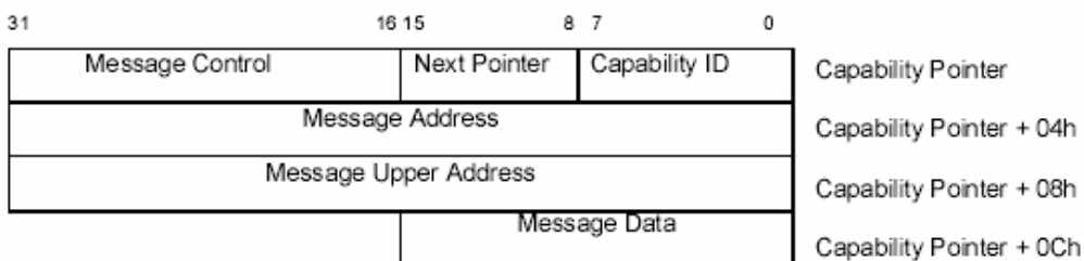
Figure 6. MSI Capability Structure
