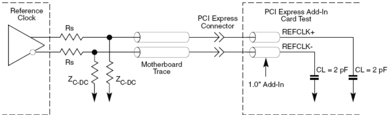
Figure 29. Reference Clock System Measurement Point and Loading
