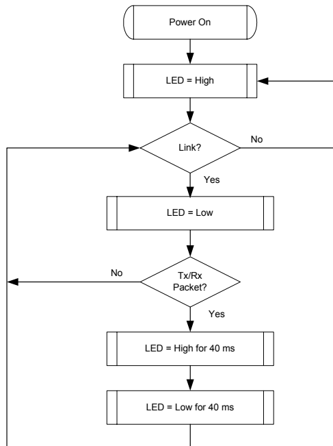
Figure 5. LINK/ACT LED
