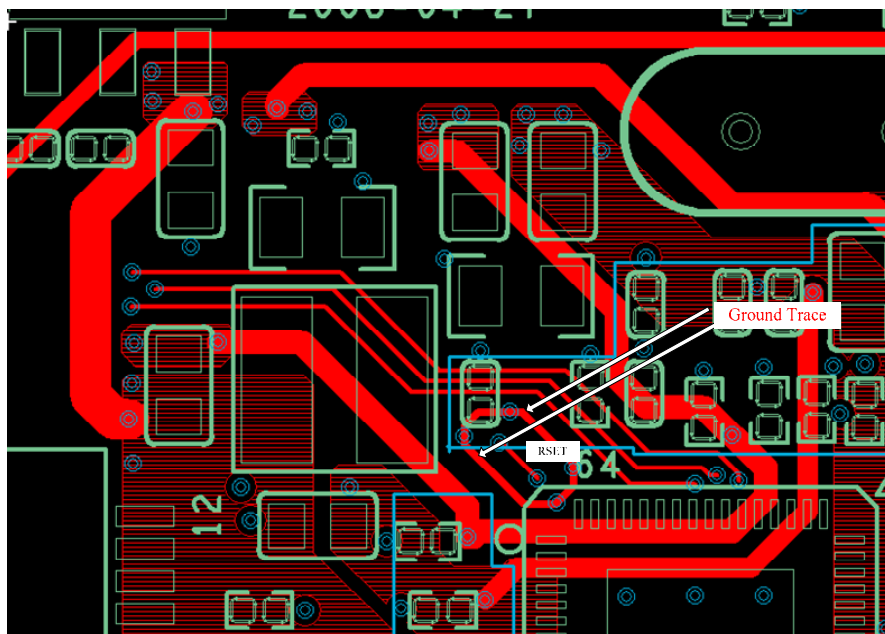
Figure 19. Typical Switching Regulator PCB Layout (Bottom Layer)
