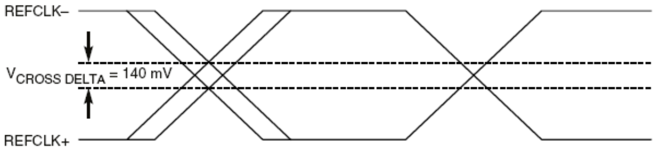
Figure 24. Single-Ended Measurement Points for Delta Cross Point
