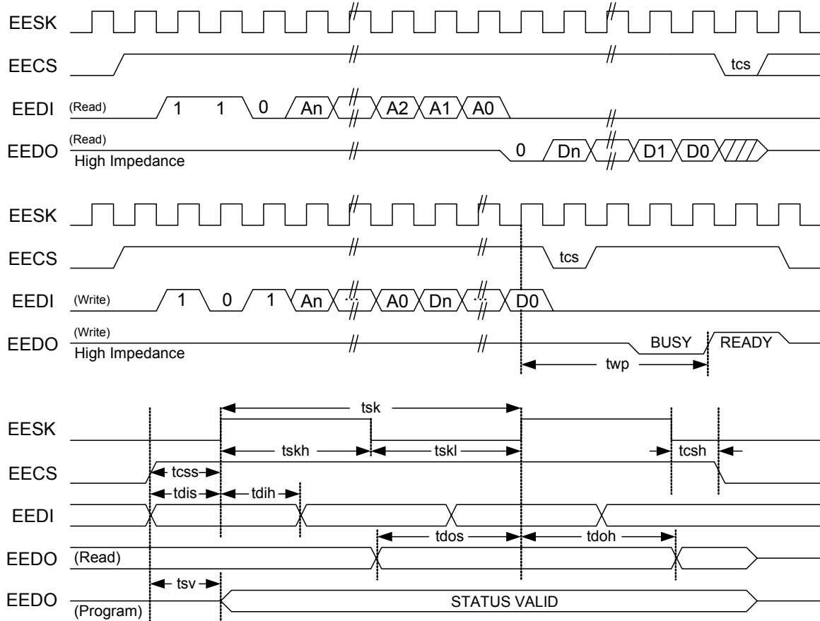
Figure 22. Serial EEPROM Interface Timing
