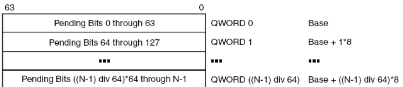
Figure 9. MSI-X PBA Structure
