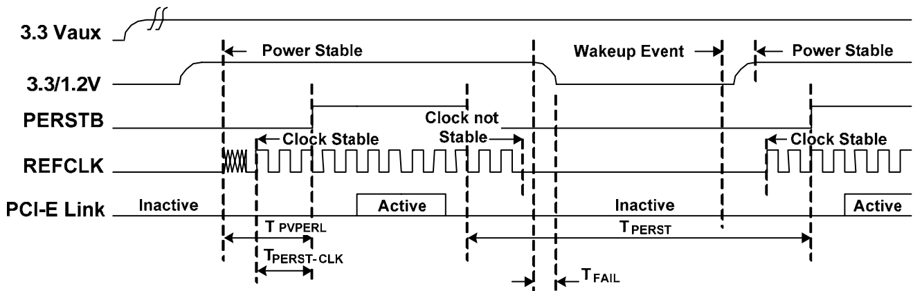
Figure 30. Auxiliary Signal Timing
