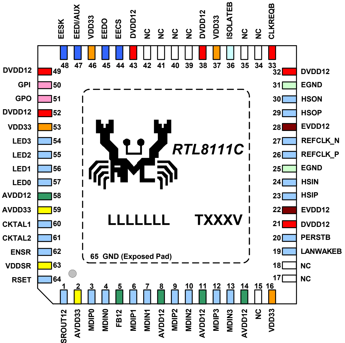
Figure 1. Pin Assignments
