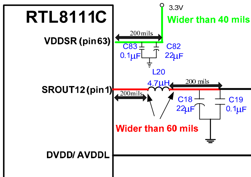
Figure 10. Switching Regulator Illustration
