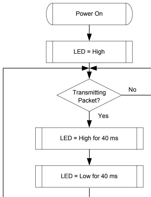
Figure 3. Tx LED
