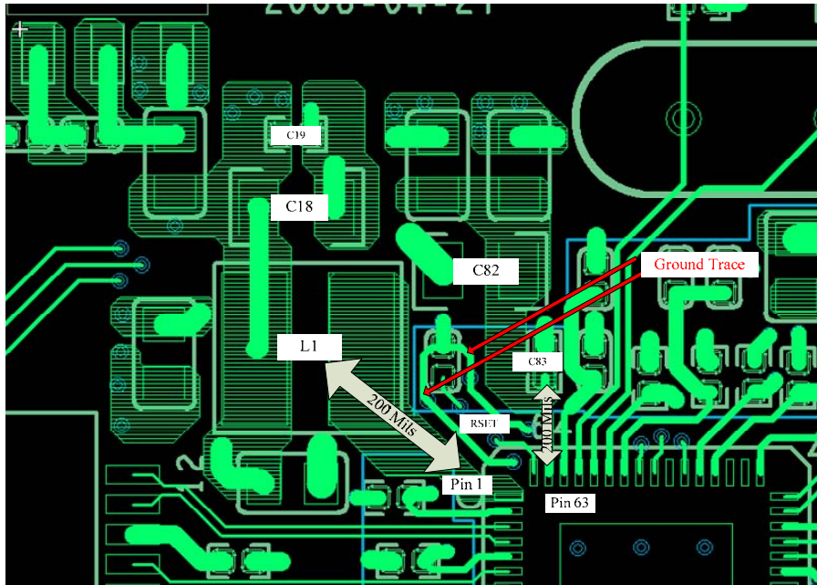
Figure 18. Typical Switching Regulator PCB Layout (Top Layer)
