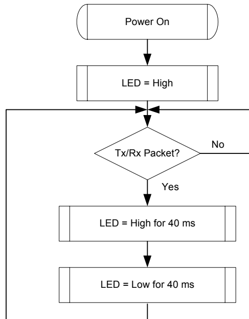
Figure 4. Tx/Rx LED
