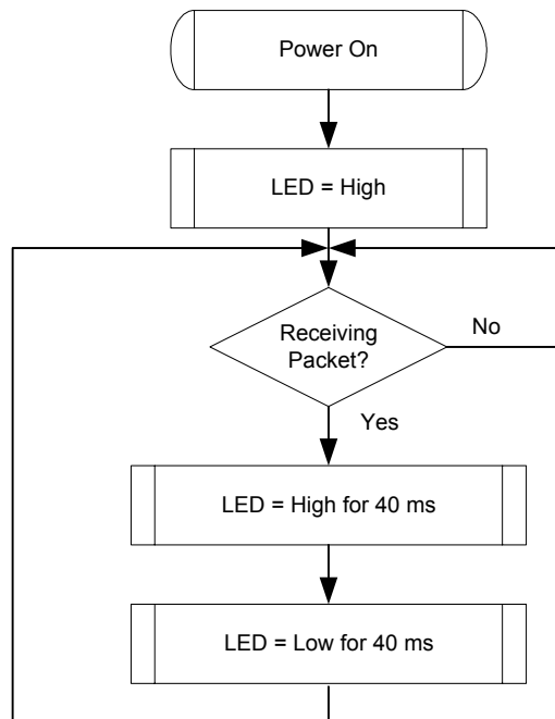
Figure 2. Rx LED
