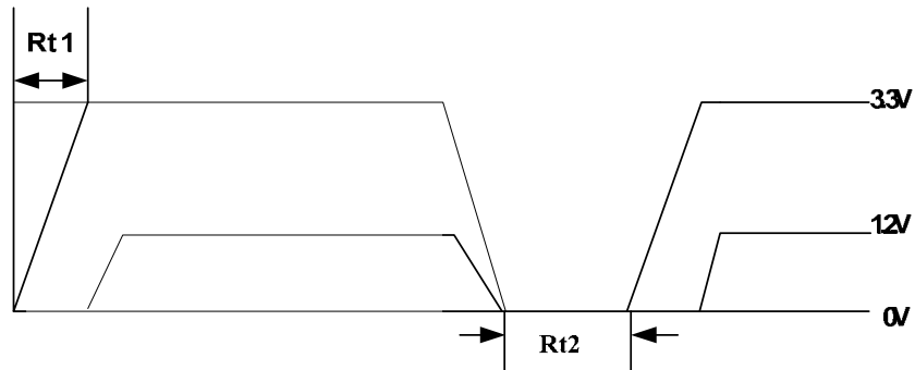
Figure 21. Power Sequence
