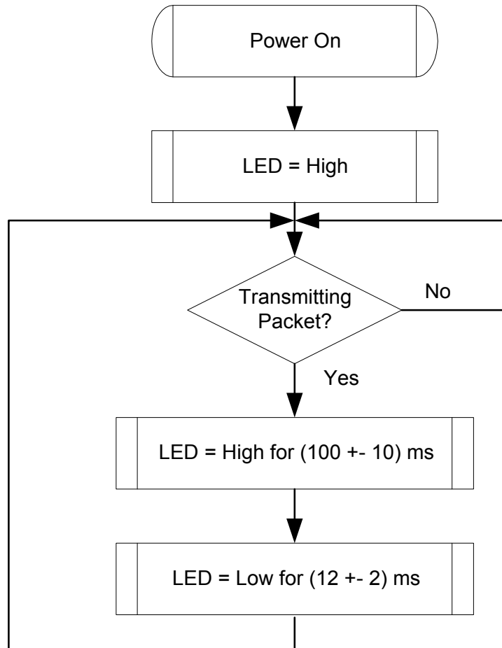
Figure 3. TX LED
