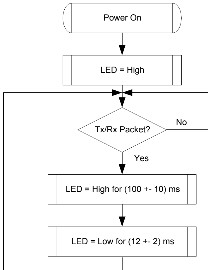
Figure 4. TX/RX LED
