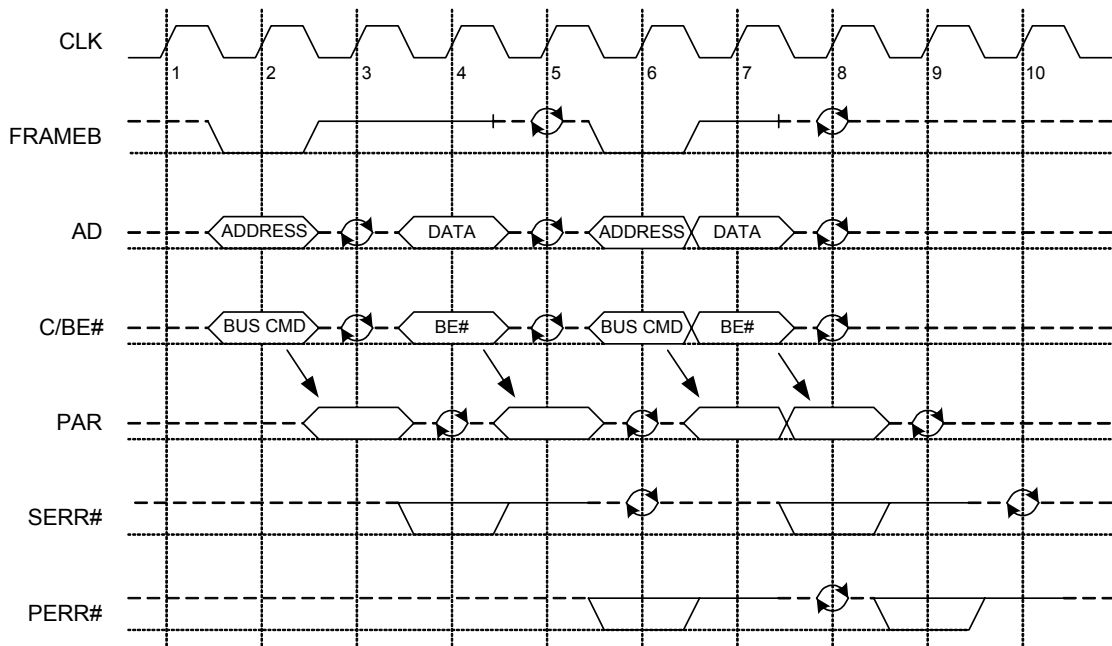
Figure 21. Parity Operation – One Example
