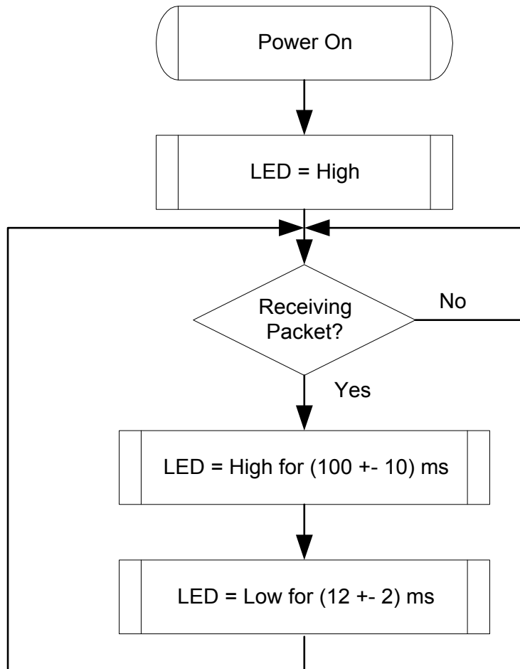
Figure 2. RX LED
