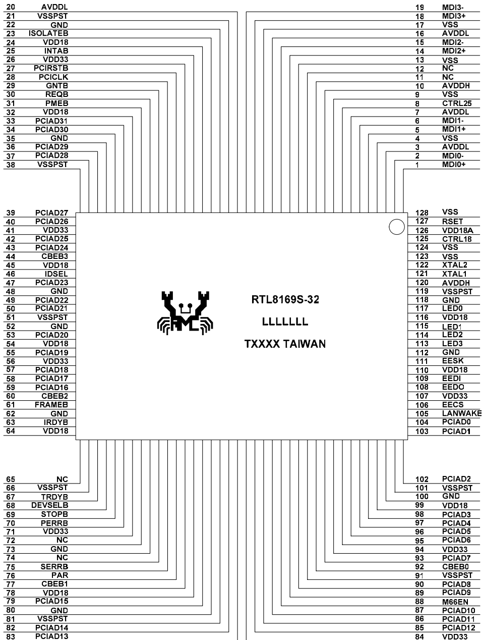
Figure 1. Pin Assignments
