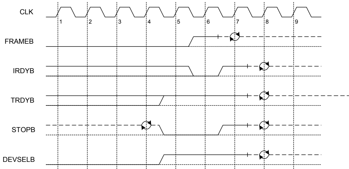
Figure 19. Target Initiated Termination - Abort
