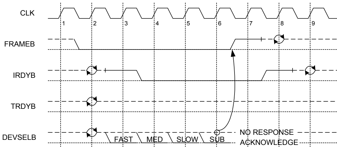
Figure 20. Master Initiated Termination - Abort
