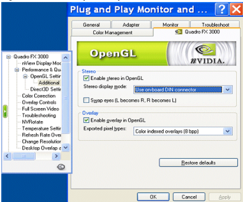
Figure 7.7 Additional OpenGL Properties — Features Enabled.
