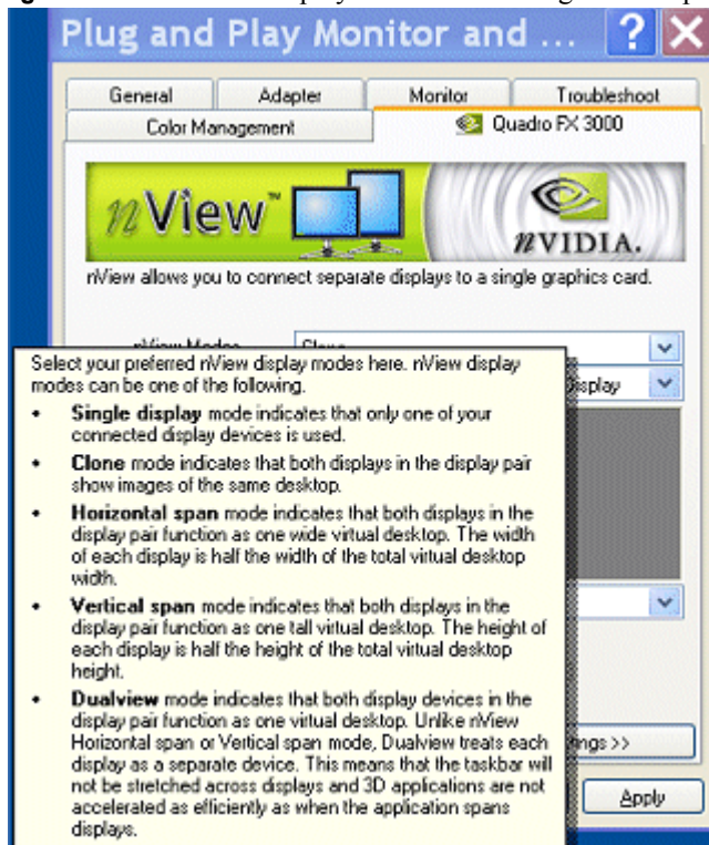
Figure 4.8 NVIDIA Display Control Panel Page — Sample Context Help
