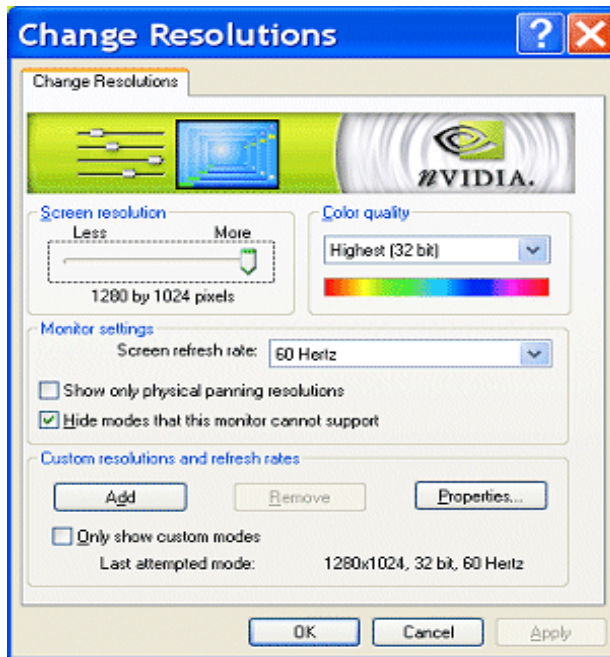
Figure 5.15 Configuring Screen Resolution for Virtual Desktop — From nView Display Modes Page
