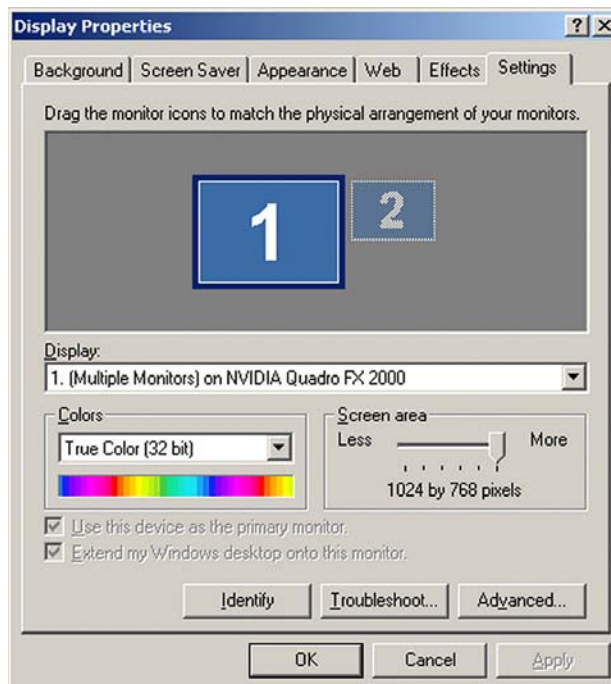
Figure 5.9 Display Properties Settings — Dualview Mode (Windows 2000)
