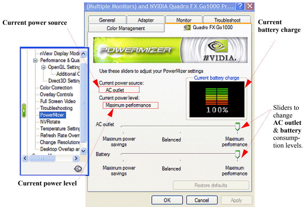
Figure 7.27 PowerMizer Settings — Applies only to Mobile Computers
