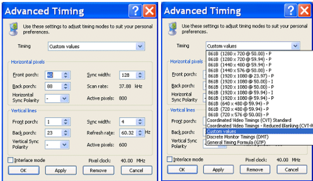
Figure 7.24 Advanced Timing Settings
