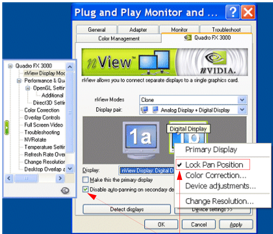
Figure 5.16 nView Clone Mode with Virtual Desktop Enabled — Disabling Panning
